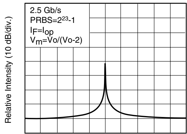
Fig. 2 Lasing Spectrum
