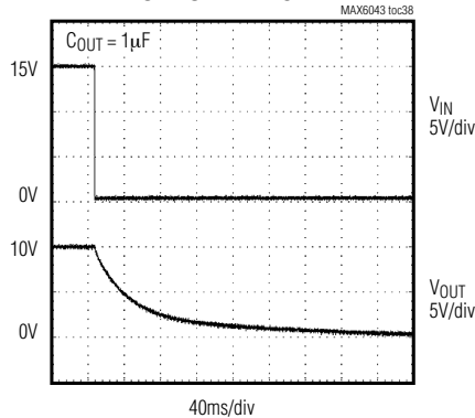
TURN-OFF TRANSIENT
