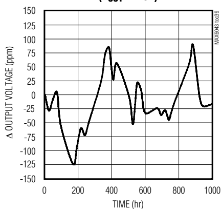
LONG-TERM DRIFT ( V_{OUT} = 2.5V )
