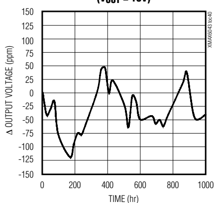
LONG-TERM DRIFT ( V_{OUT} = 10V )
