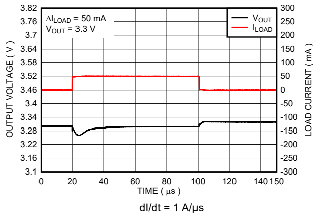
Figure 7-14. Load Transient Response (New Chip)
