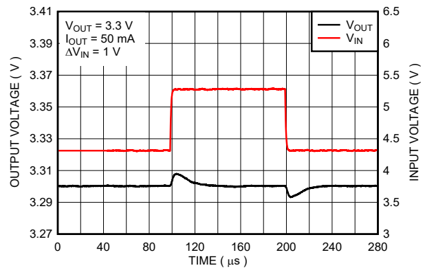
Figure 5-20. Line Transient Response (Legacy Chip)
