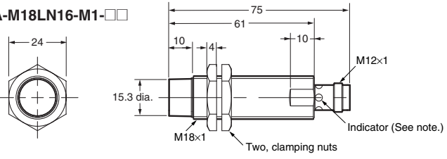
E2A-M18LN16-M1-□□
