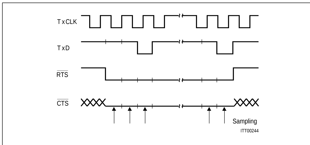
Figure 31 RTS-CTS Handshaking
