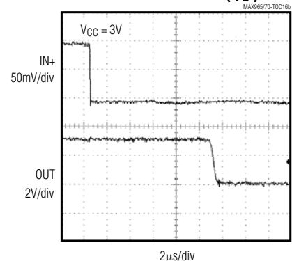
PROPAGATION DELAY ( t_{PD-} )
