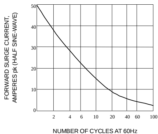
Fig. 4-NON-RECURRENT SURGE RATING
