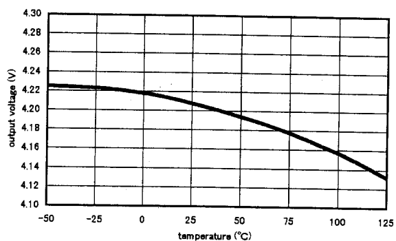
RESET detecting voltage Temperature Characteristic
