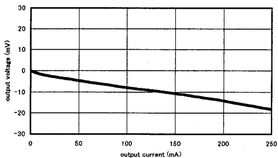
Load Regulation
