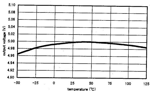
Regulator Output voltage Temperature Characteristic
