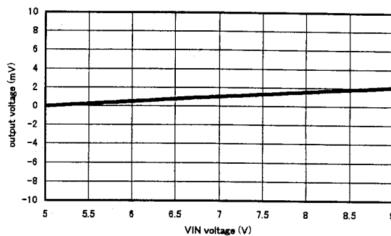
Line Regulation
