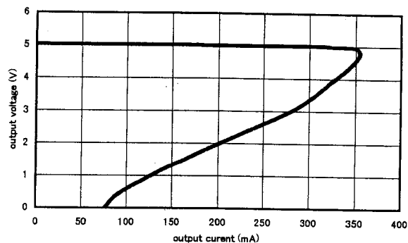
Current Limit
