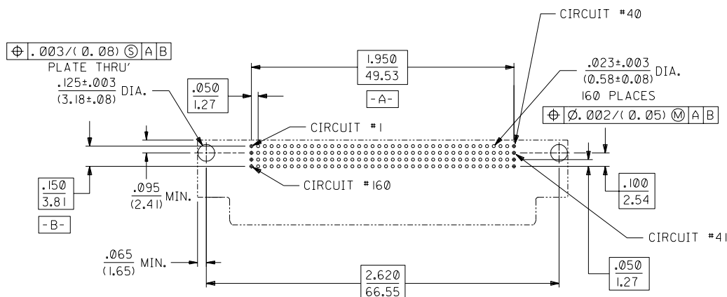
RECOMMENDED PC BOARD LAYOUT COMPONENT SIDE
