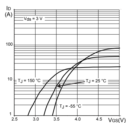
Figure 6. Transfer characteristics
