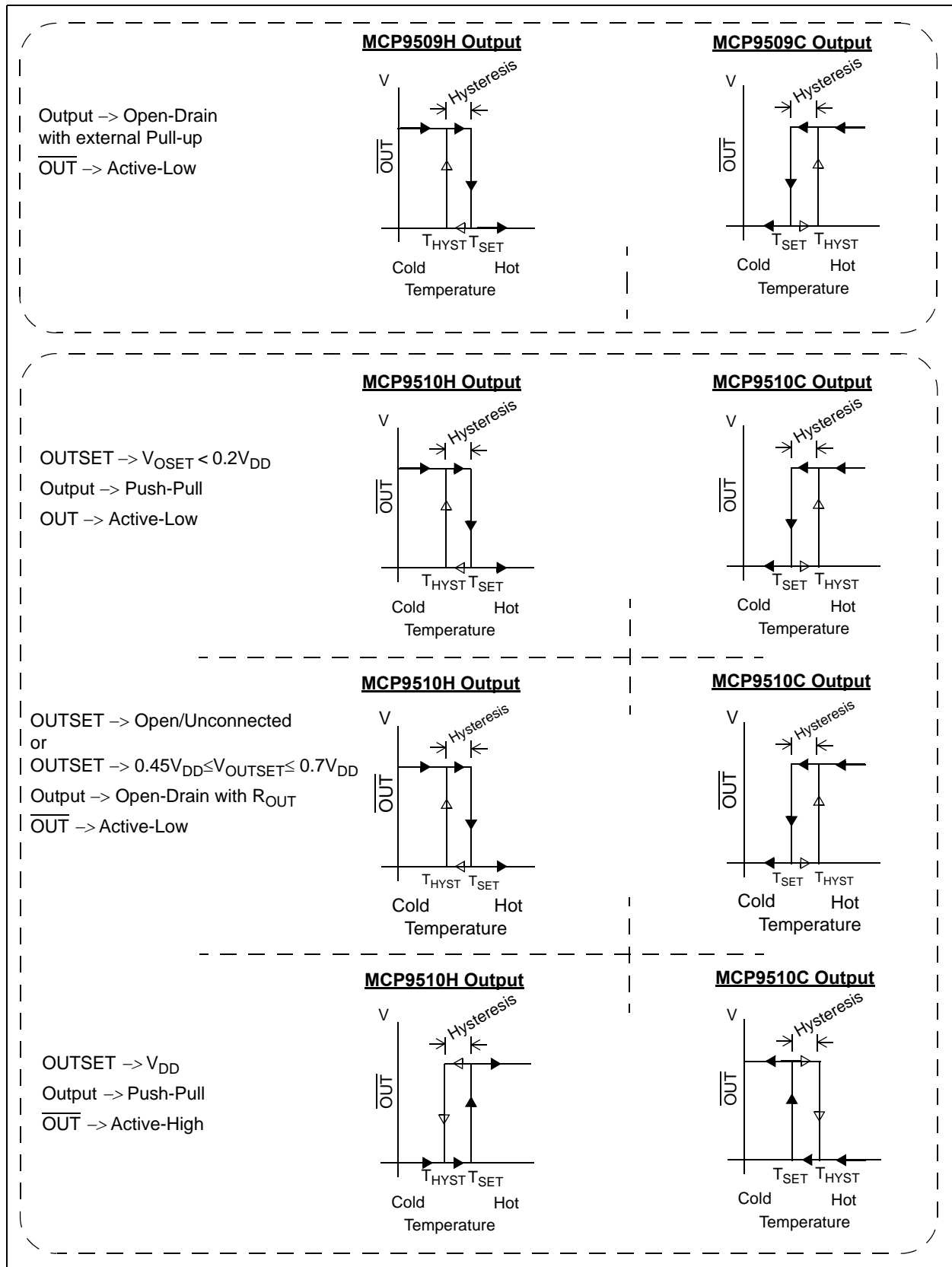
FIGURE 4-4: MCP9509/10 \text{OUT}/\overline{\text{OUT}} Output Configuration.
