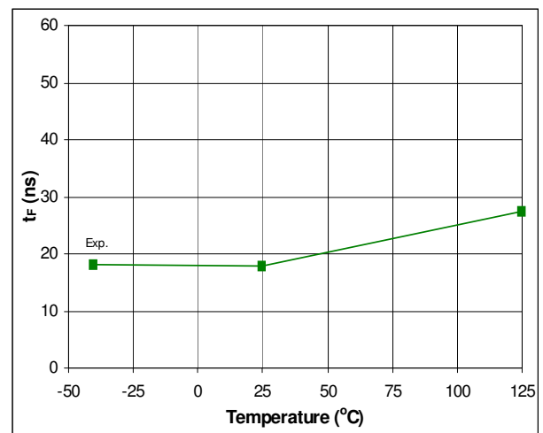
Fig. 27. Turn-off Fall Time vs. Temperature
