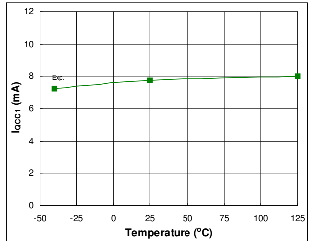
Fig. 31. Quiescent VCC Supply Current vs. Temperature
