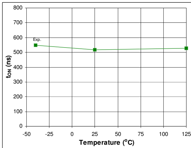
Fig. 24. Turn-on Propagation Delay vs. Temperature
