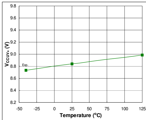
Fig. 36. VCC Supply Under-voltage Positive Going Threshold vs. Temperature
