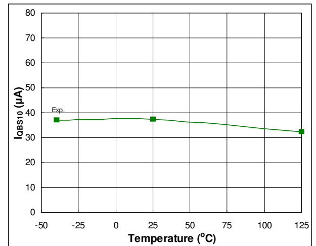
Fig. 33. Quiescent VBS Supply Current vs. Temperature
