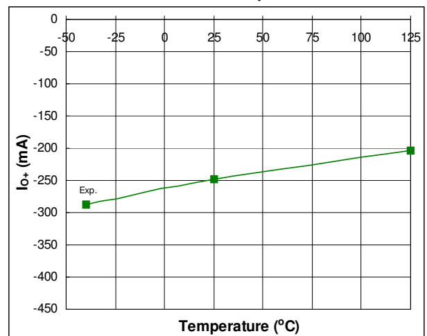
Fig. 39. Output High Short Circuit Pulsed Current vs. Temperature
