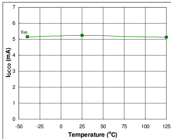
Fig. 32. Quiescent VCC Supply Current vs. Temperature
