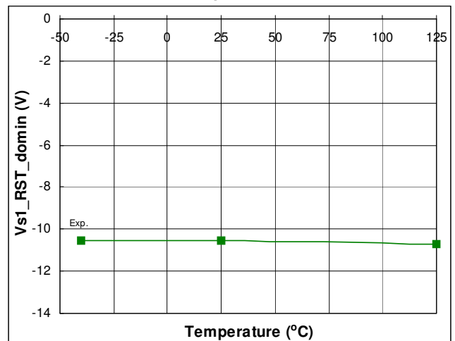
Fig. 41. Max -Vs vs. Temperature
