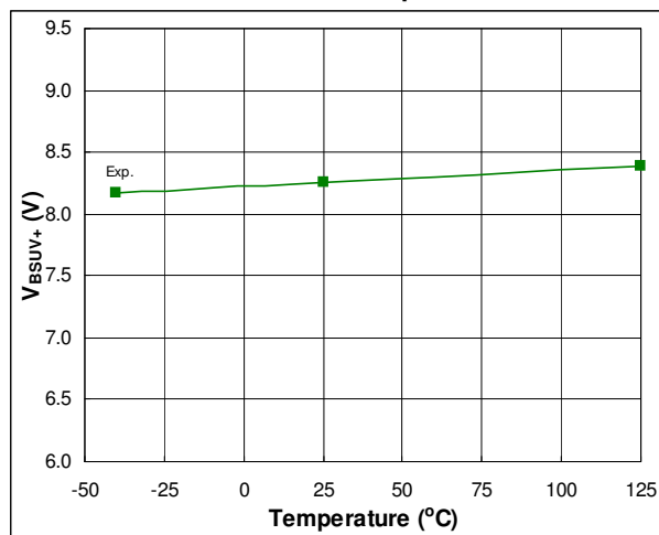
Fig. 38. VBS Supply Under-voltage Positive Going Threshold vs. Temperature
