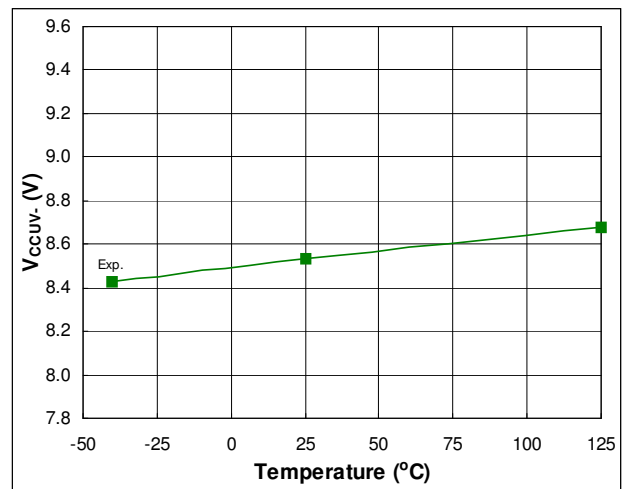
Fig. 35. VCC Supply Under-voltage Negative Going Threshold vs. Temperature
