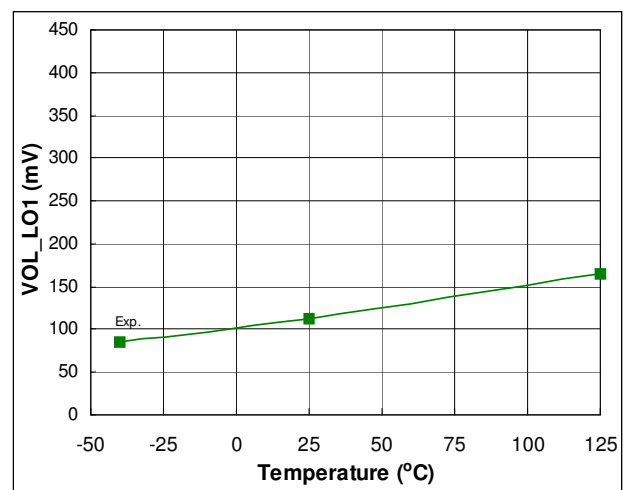
Fig. 29. Low Level Output Voltage vs. Temperature
