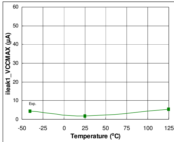
Fig. 30. Offset Supply Leakage Current vs. Temperature
