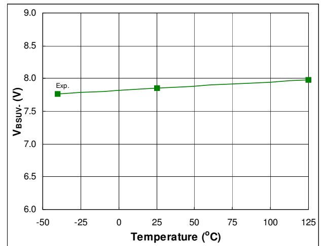
Fig. 37. VBS Supply Under-voltage Negative Going Threshold vs. Temperature
