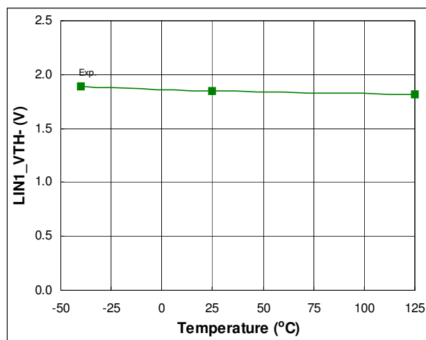
Fig. 28. Input Negative Going Threshold vs. Temperature
