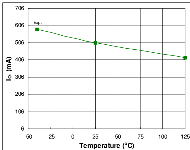
Fig. 40. Output Low Short Circuit Pulsed Current vs. Temperature
