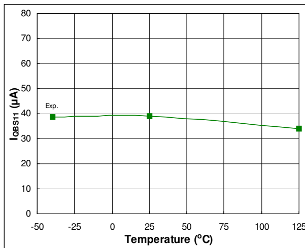
Fig. 34. Quiescent VBS Supply Current vs. Temperature
