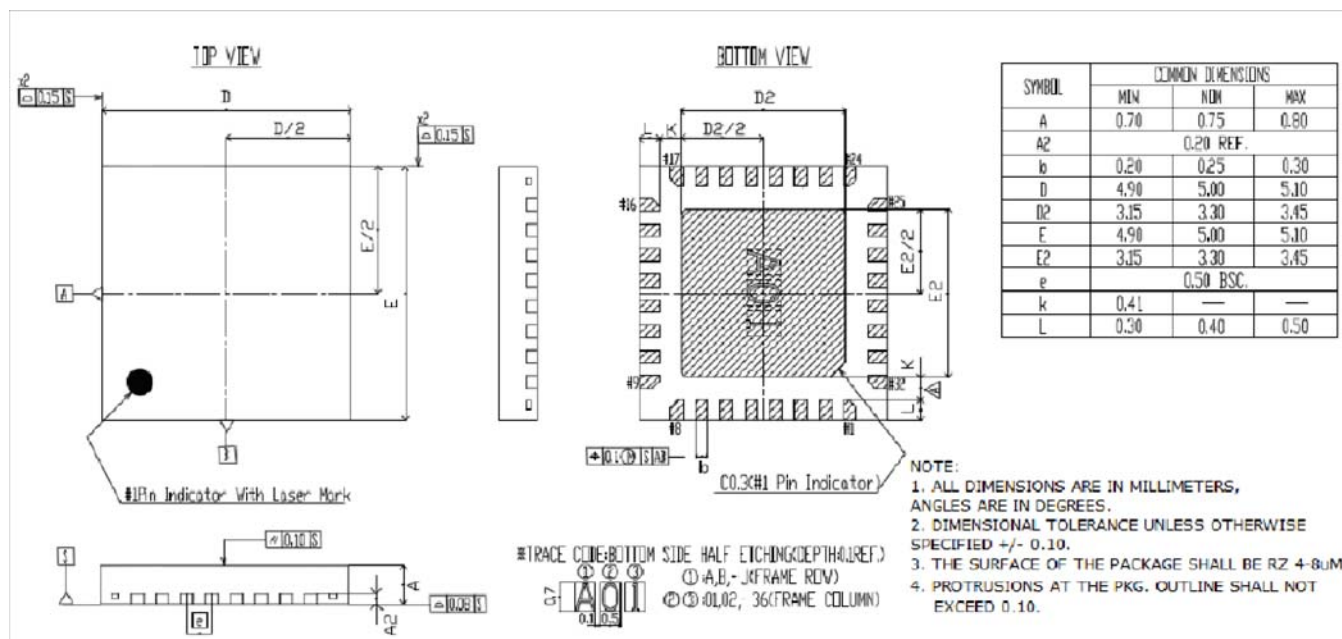
32-Lead OFN 5x 5mm
