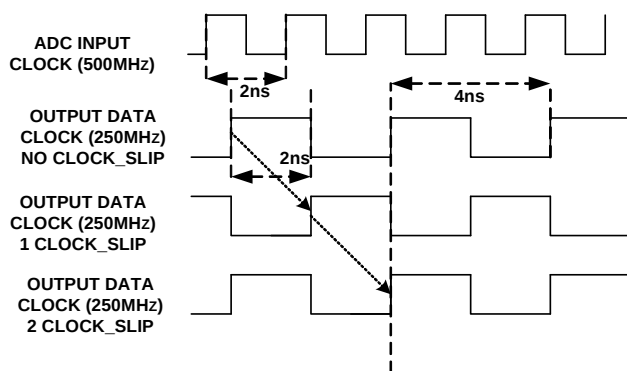
FIGURE 42. PHASE SLIP
