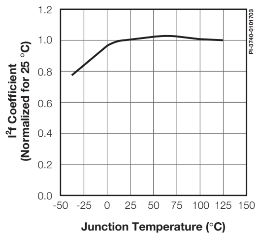
Figure 22. I^2f Coefficient vs. Temperature.
