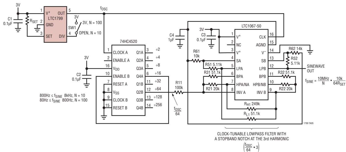
Low Power 80Hz to 8kHz Sine Wave Generator ( I_Q < 4\text{mA} )
