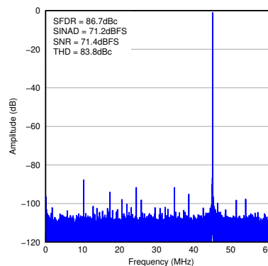
Figure 7-29. FFT for 170-MHz Input Signal
