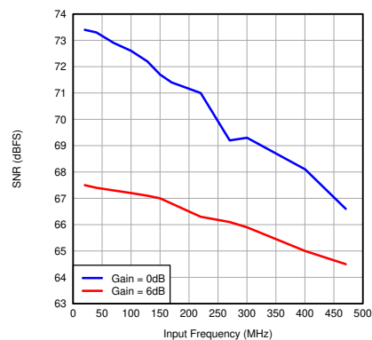
Figure 7-33. SNR vs Input Frequency
