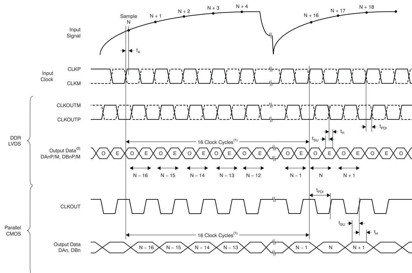
Figure 7-1. CMOS Interface Timing Diagram
