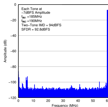
Figure 7-31. FFT for Two-Tone Input Signal
