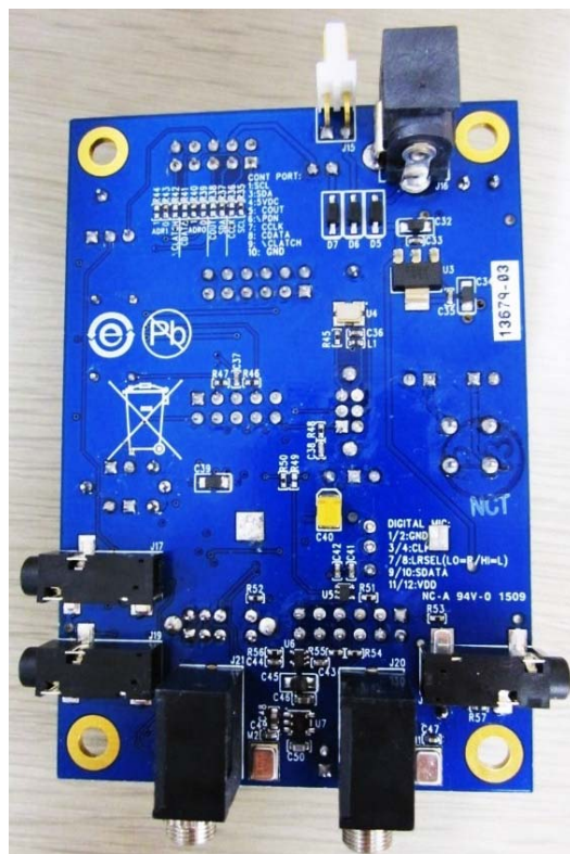
Figure 2. Evaluation Board Bottom Side
