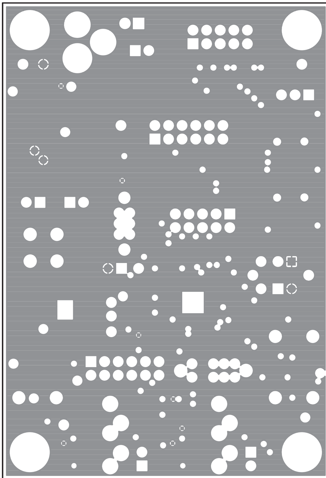
Figure 46. Evaluation Board Layout—Power Plane
