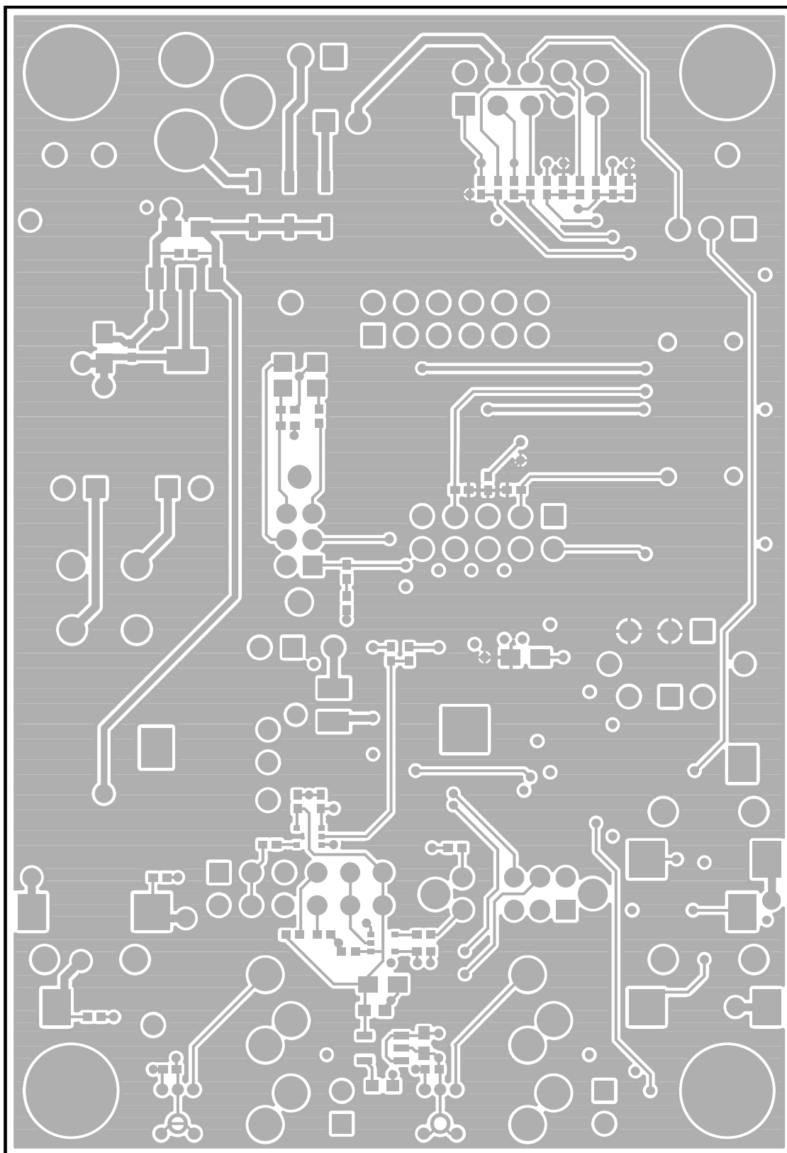
Figure 48. Evaluation Board Layout—Bottom Copper
