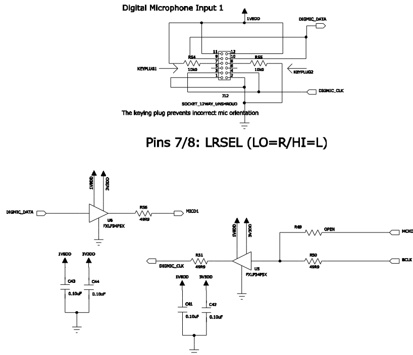
Figure 39. Evaluation Board Schematic—Digital Microphone Interface
