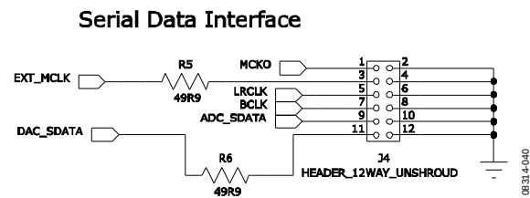
Figure 40. Evaluation Board Schematic—Serial Audio Data Interface
