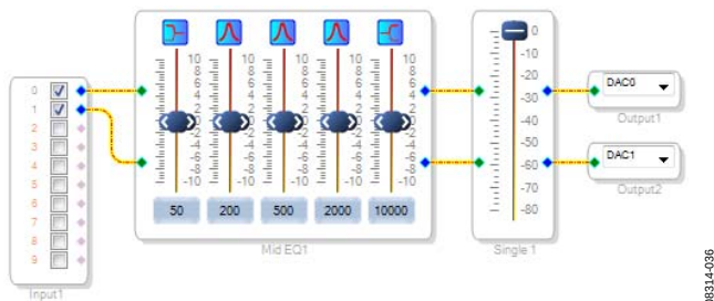
Figure 36. Completed Signal Flow
