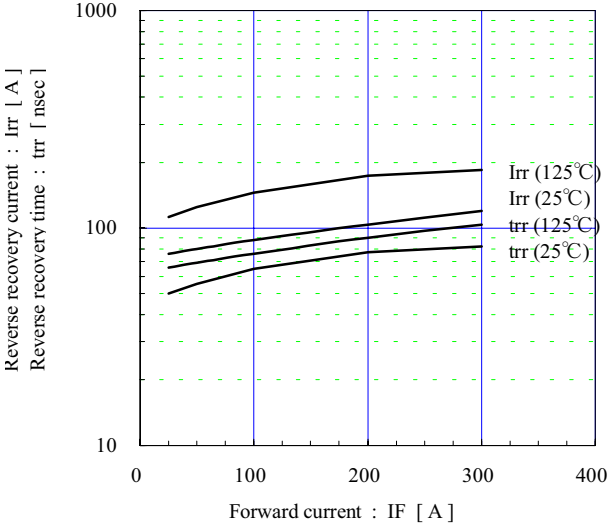
Reverse recovery characteristics (typ.) Vcc=300V, VGE=±15V, Rg=16Ω
