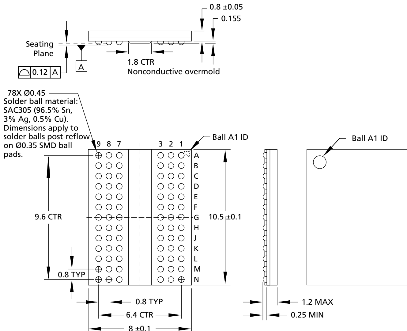
Figure 3: 78-Ball FBGA – x4, x8 (DA)
