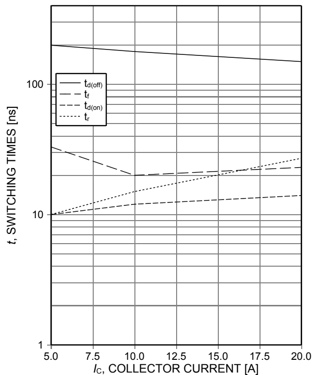
Figure 9. Typical switching times as a function of collector current (inductive load, T_{vj}=175^{\circ}\text{C} , V_{CE}=400\text{V} , V_{GE}=15/0\text{V} , r_G=26\Omega , Dynamic test circuit in Figure E)
