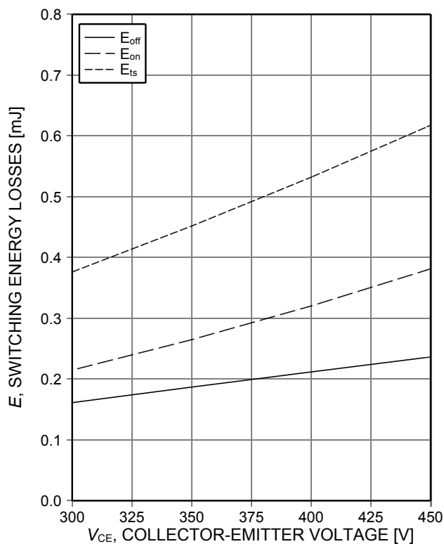
Figure 16. Typical switching energy losses as a function of collector emitter voltage (inductive load, T_{vj}=175^\circ\text{C} , V_{GE}=15/0\text{V} , I_C=10\text{A} , r_G=26\Omega , Dynamic test circuit in Figure E)
