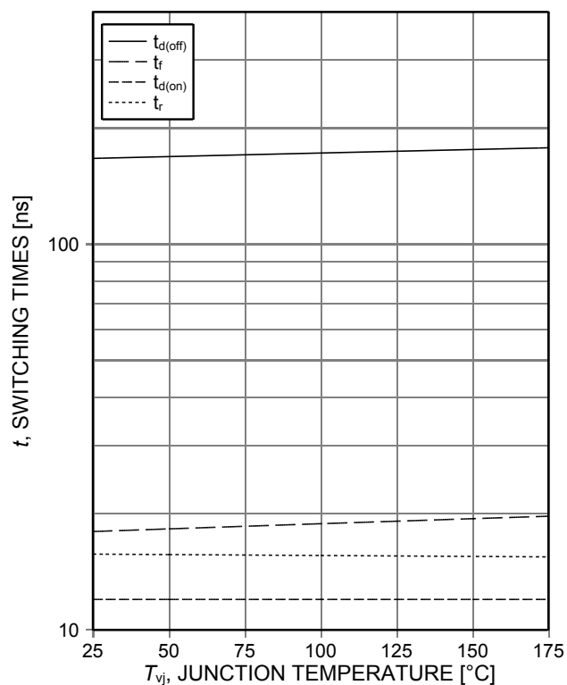
Figure 11. Typical switching times as a function of junction temperature (inductive load, V_{CE}=400\text{V} , V_{GE}=15/0\text{V} , I_C=10\text{A} , r_G=26\Omega , Dynamic test circuit in Figure E)
