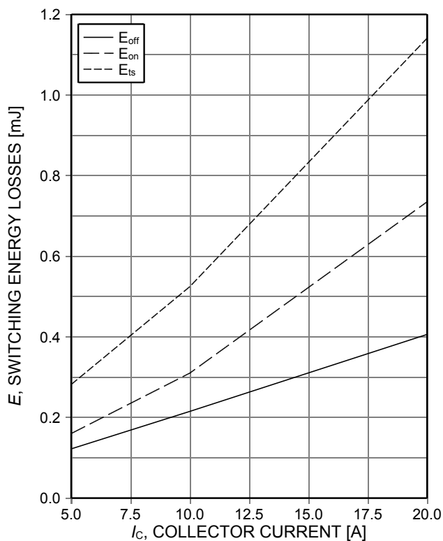
Figure 13. Typical switching energy losses as a function of collector current (inductive load, T_{vj}=175^\circ\text{C} , V_{CE}=400\text{V} , V_{GE}=15/0\text{V} , r_G=26\Omega , Dynamic test circuit in Figure E)
