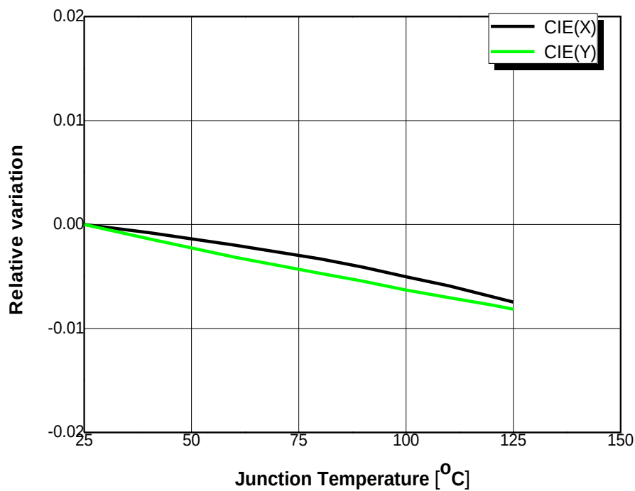
Fig 7. Junction Temp. vs. CIE X, Y Shift, IF=1000mA (Warm white)
