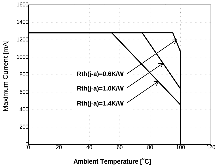
Fig 8. Maximum Forward Current vs. Ambient Temperature, T_j(\text{max.}) = 125^\circ\text{C} , I_F = 1.28\text{A}
