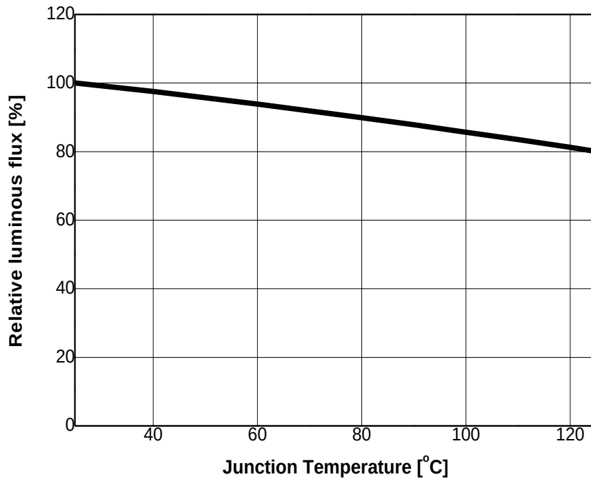
Fig 6. Relative Light Output vs. Junction Temperature, IF=1000mA
