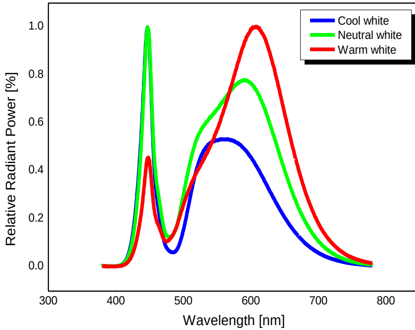
Fig 1. Color Spectrum, Ta = 25℃, IF = 1000mA, RH30%
