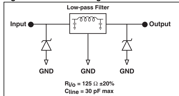
Figure 2. Device configuration
