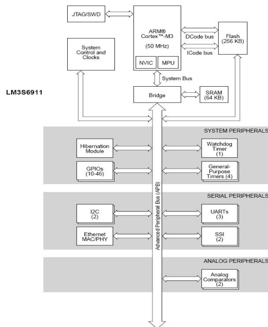
Figure 2 LM3S6911 Block Diagram
