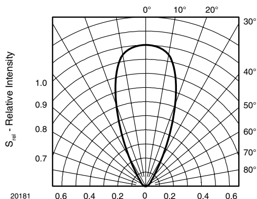
Fig. 3 - Relative Radiant Sensitivity vs. Angular Displacement
