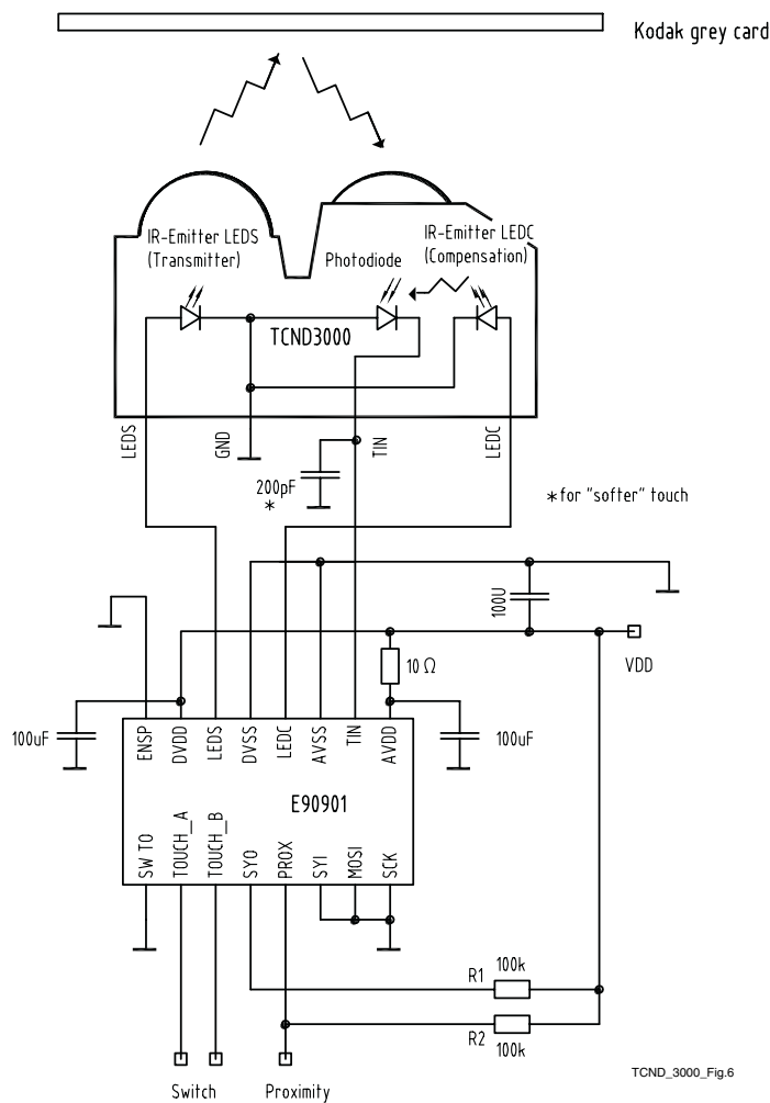
Fig. 6 - Test Circuit
