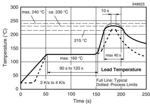
Fig. 8 - Lead (Pb)-free Reflow Solder Profile acc. J-STD-020
