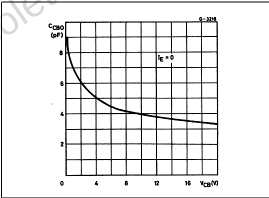
Figure 3. Collector-base capacitance
