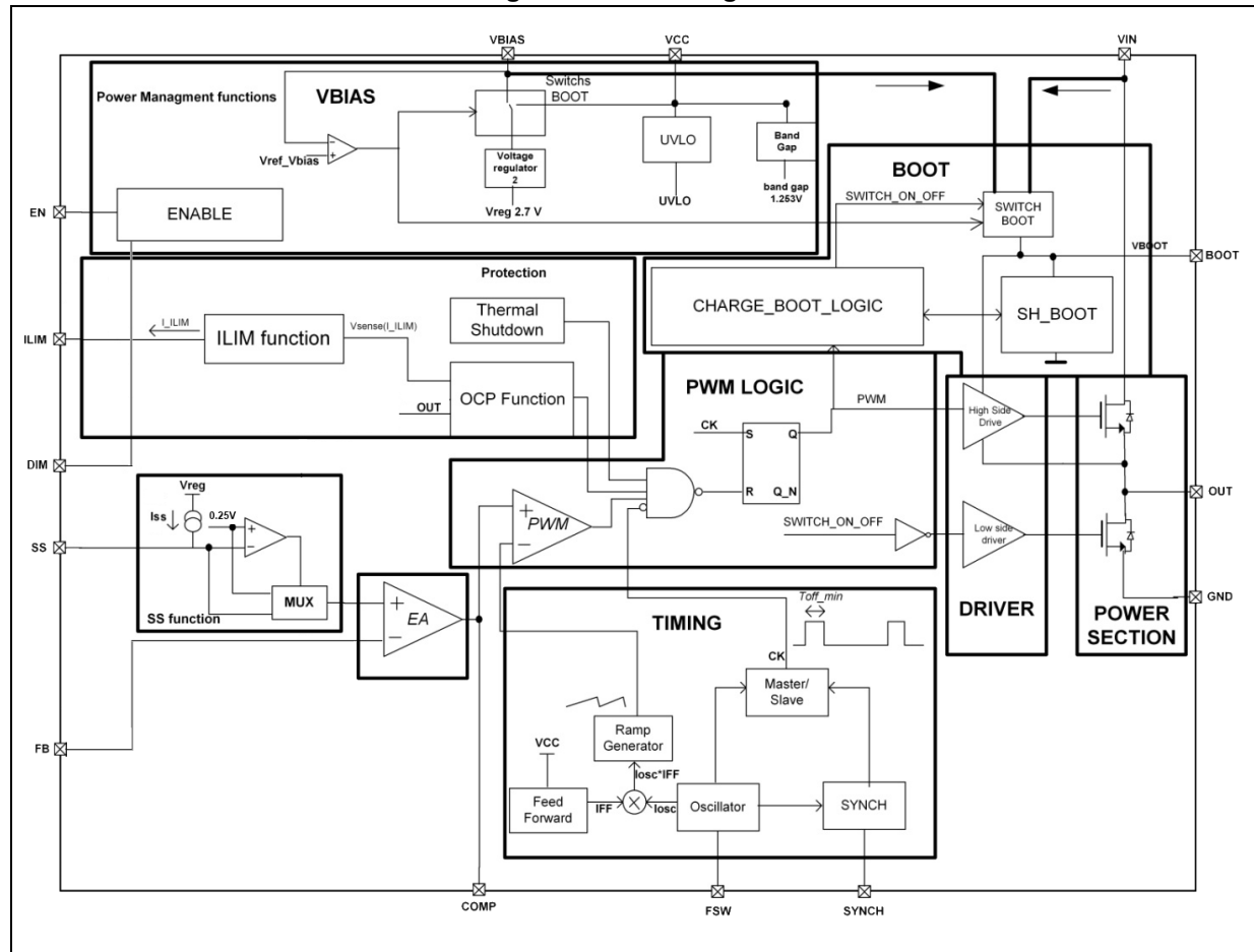
Figure 2. Block diagram
