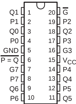
54ACT11520 . . . J PACKAGE 74ACT11520 . . . DW OR N PACKAGE (TOP VIEW)
