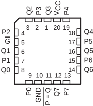
54ACT11520 . . . FK PACKAGE (TOP VIEW)
