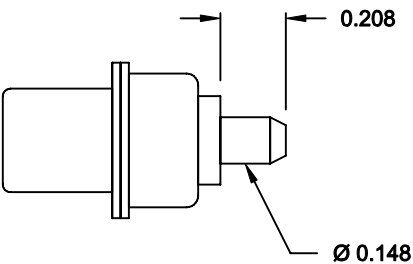
POWER CONTACTS
