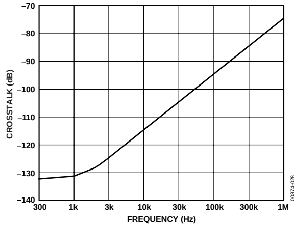
Figure 28. Crosstalk vs. Frequency
