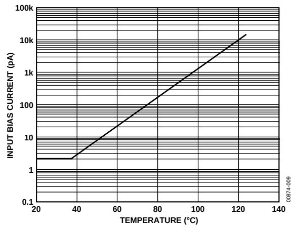
Figure 9. Input Bias Current vs. Temperature; V_S = 5V, V_{CM} = 0
