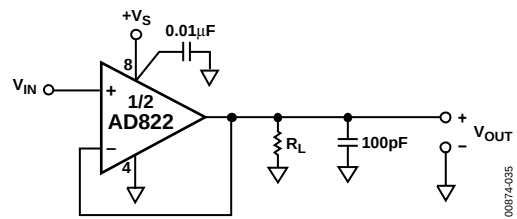
Figure 35. Unity Gain Follower
