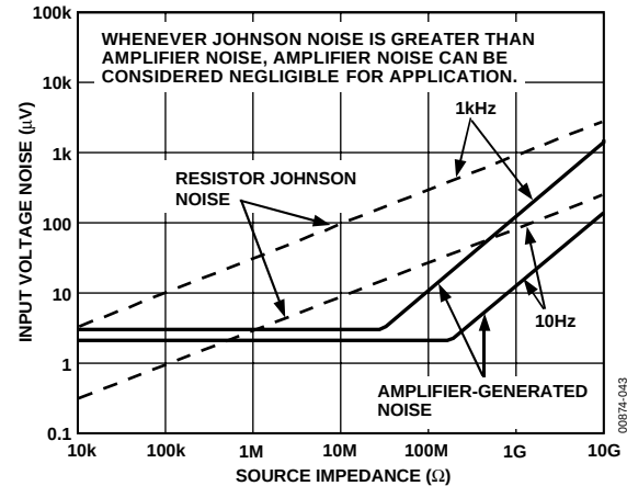
Figure 43. Total Noise vs. Source Impedance
