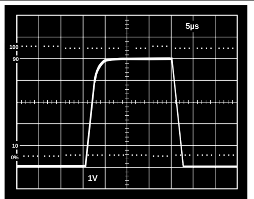
Figure 48. Pulse Response of In Amp to a 500 mV p-p Input Signal; V_S = 5\text{ V} , 0\text{ V} ; Gain = 0
