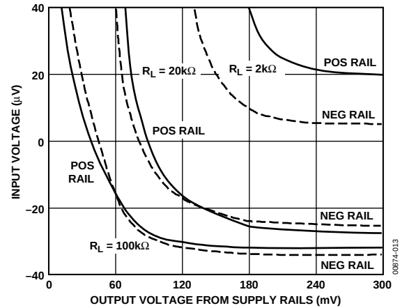
Figure 13. Input Effort Voltage with Output Voltage Within 300 mV of Either Supply Rail for Various Resistive Loads; V_S = \pm 5\text{ V}
