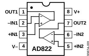
Figure 1. 8-Lead PDIP (N Suffix); 8-Lead MSOP (RM Suffix); and 8-Lead SOIC (R Suffix)
