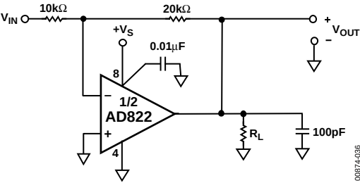
Figure 36. Gain-of-T2 Inverter
