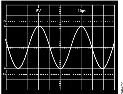
Figure 30. 20 V p-p, 25 kHz Sine Wave Input; Unity Gain Follower; R_L = 600 \Omega , V_S = \pm 15 \text{ V}
