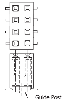
Two Row SMT, With Guide Post (P)
