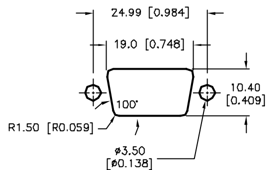
Panel Cutout
