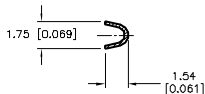
SECTION B
