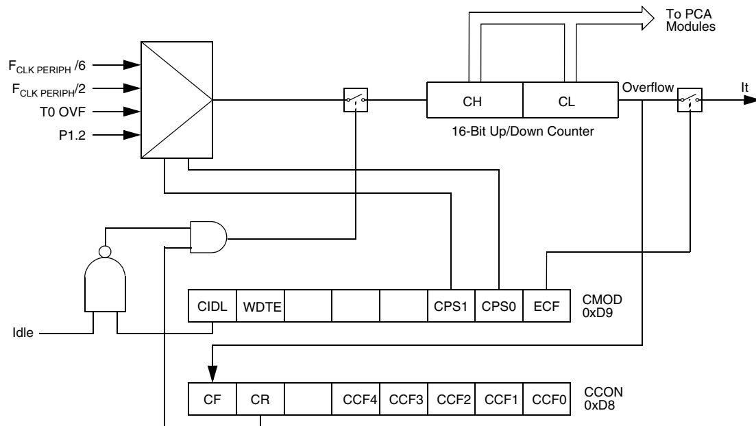
Figure 10-1. PCA Timer/Counter
