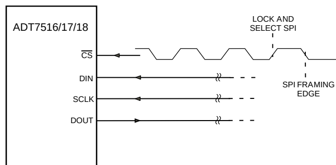
Figure 23(b). Typical SPI Interface Connection
