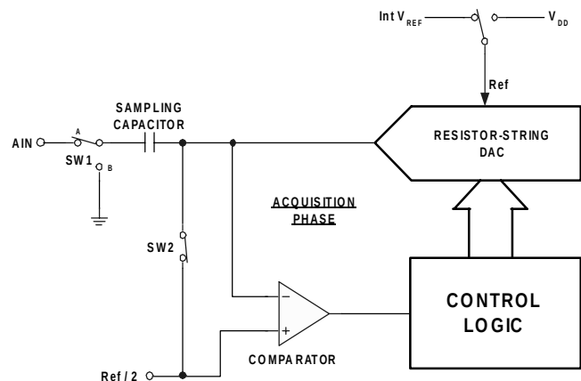
Figure 14. ADC Acquisition Phase
