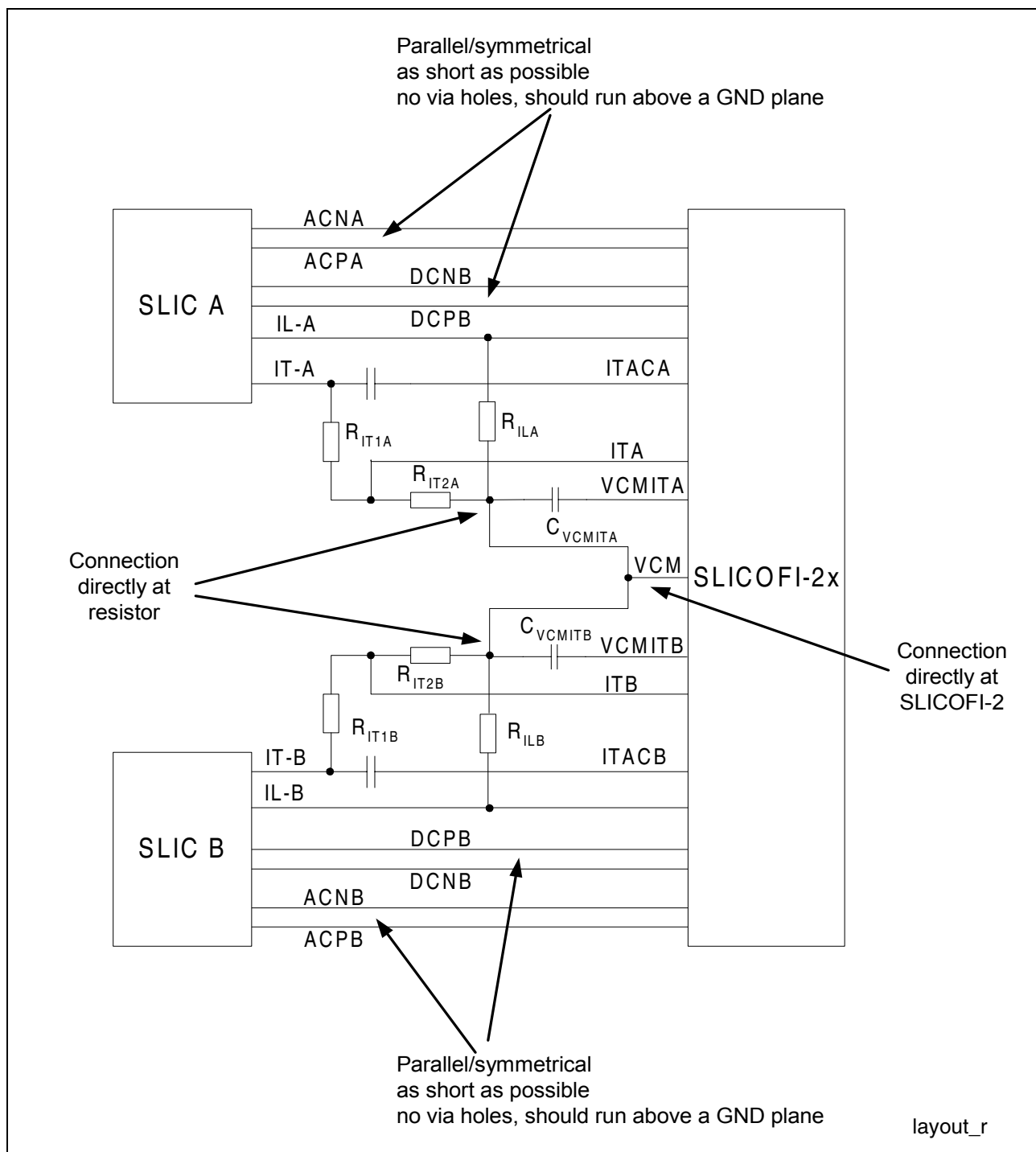
Figure 96 DuSLIC Layout Recommendation
