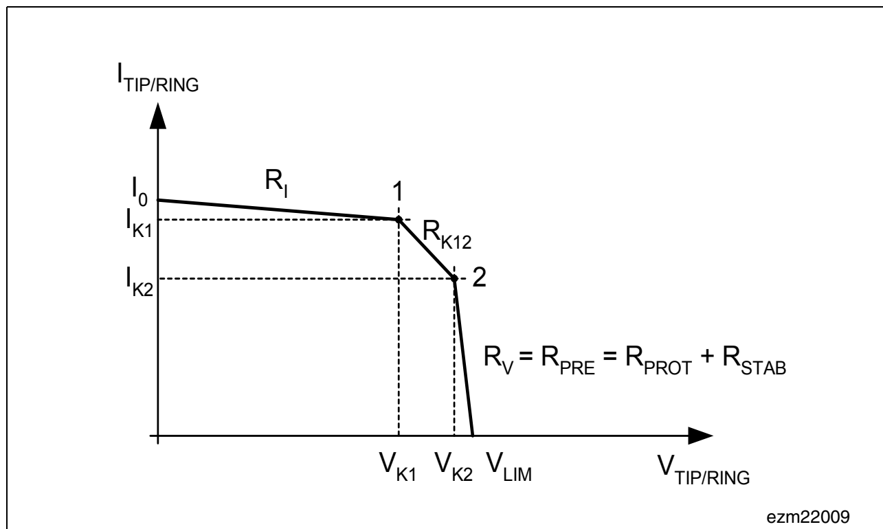
Figure 15 DC Characteristics
