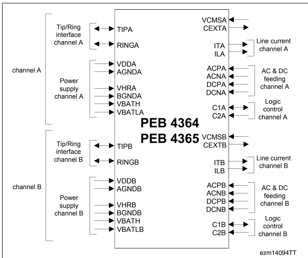
Figure 6 Logic Symbol: TSLIC-S/TSLIC-E
