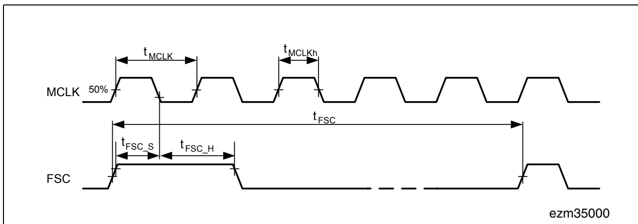
Figure 84 MCLK/FSC-Timing
