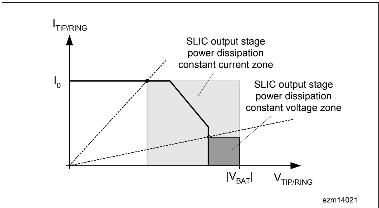
Figure 16 Power Dissipation
