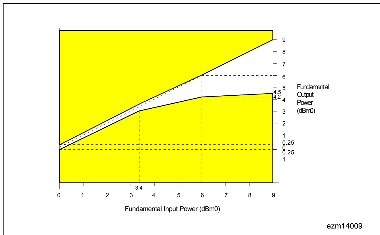
Figure 72 Overload Compression
