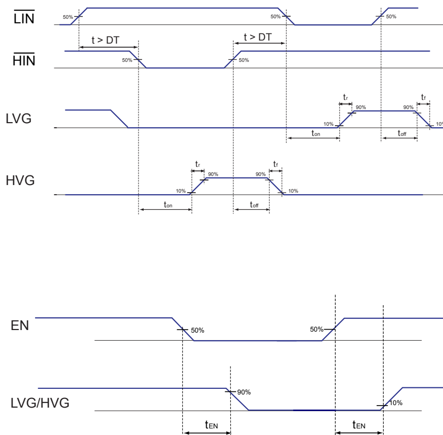
Figure 5. Deadtime timing definitions
