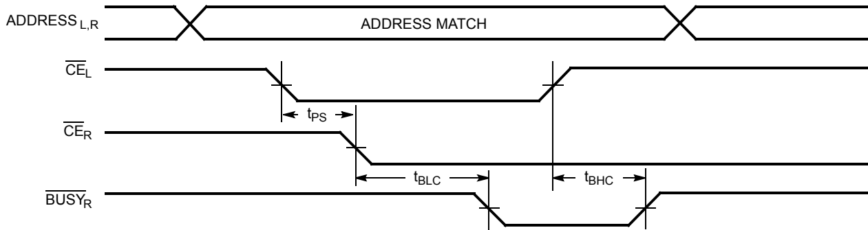
Figure 14. Busy Timing Diagram No.1 ( \overline{\text{CE}} Arbitration) [47]
