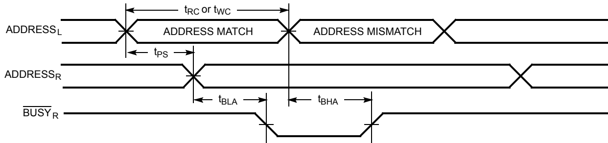
Figure 15. Busy Timing Diagram No.2 (Address Arbitration) [47]
