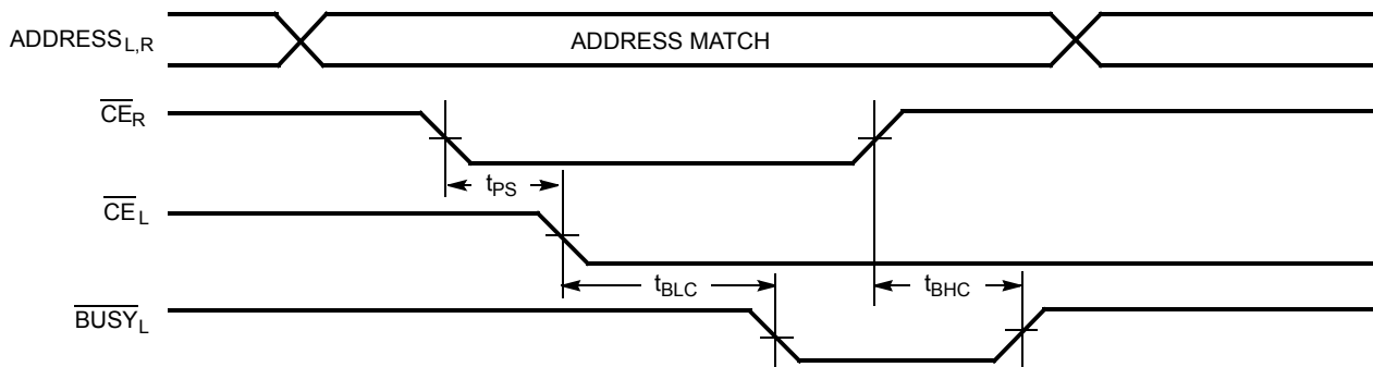
Figure 15. Busy Timing Diagram No.2 (Address Arbitration) [47]
