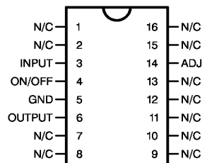
16-Lead Ceramic Dual-in-Line Package
