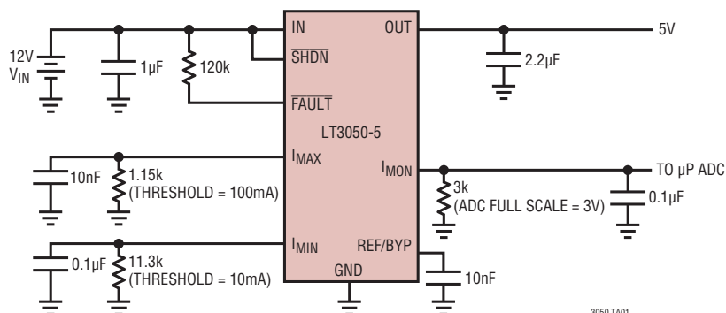
5V Supply with 100mA Precision Current Limit, 10mA I_{\text{MIN}}
