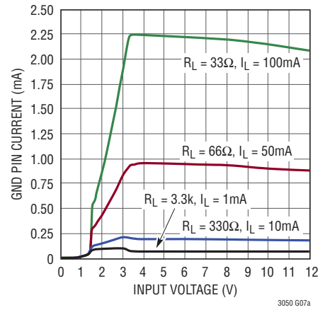
GND Pin Current LT3050-3.3
