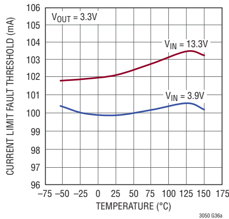
External Current Limit R_{I\text{MAX}} = 1.15\text{k}
