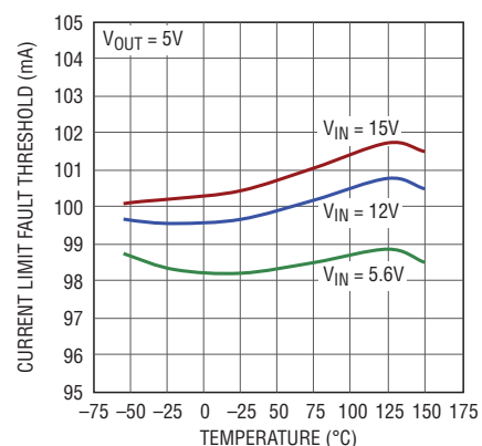
External Current Limit R_{\text{IMAX}} = 1.15\text{k}
