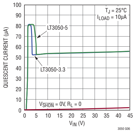
Quiescent Current
