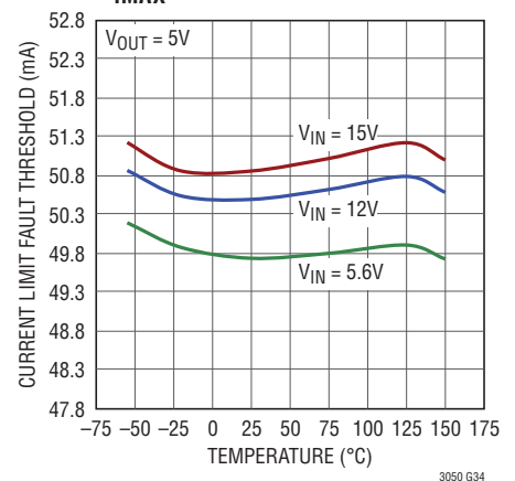
External Current Limit R_{I\text{MAX}} = 2.26\text{k}
