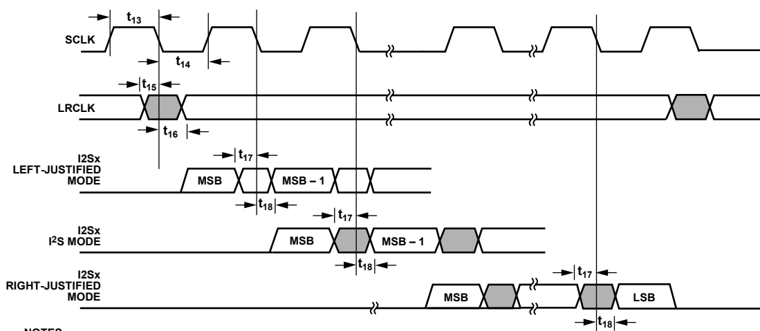
Figure 4. I²S Timing
