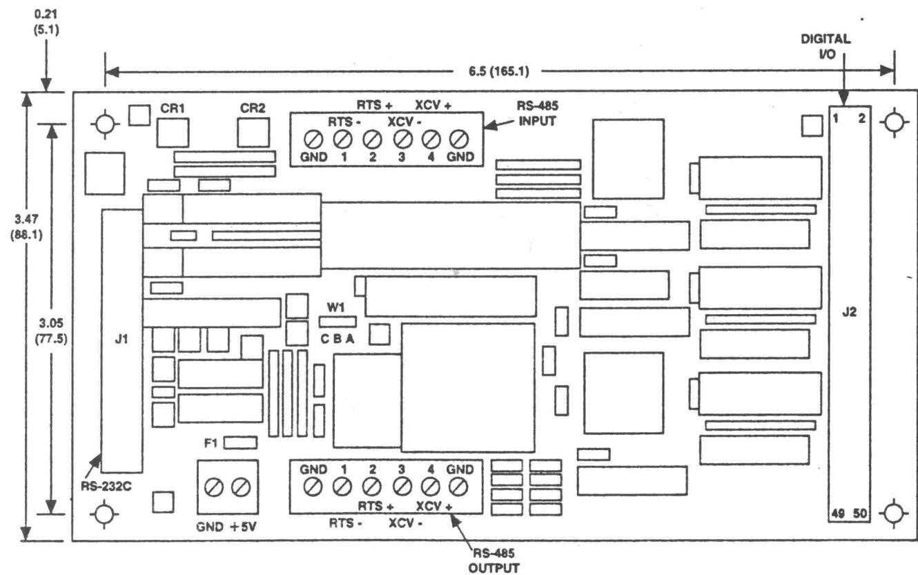
Figure 5. Outline Dimensions
