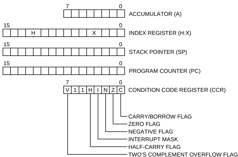
Figure 10-1. CPU registers
