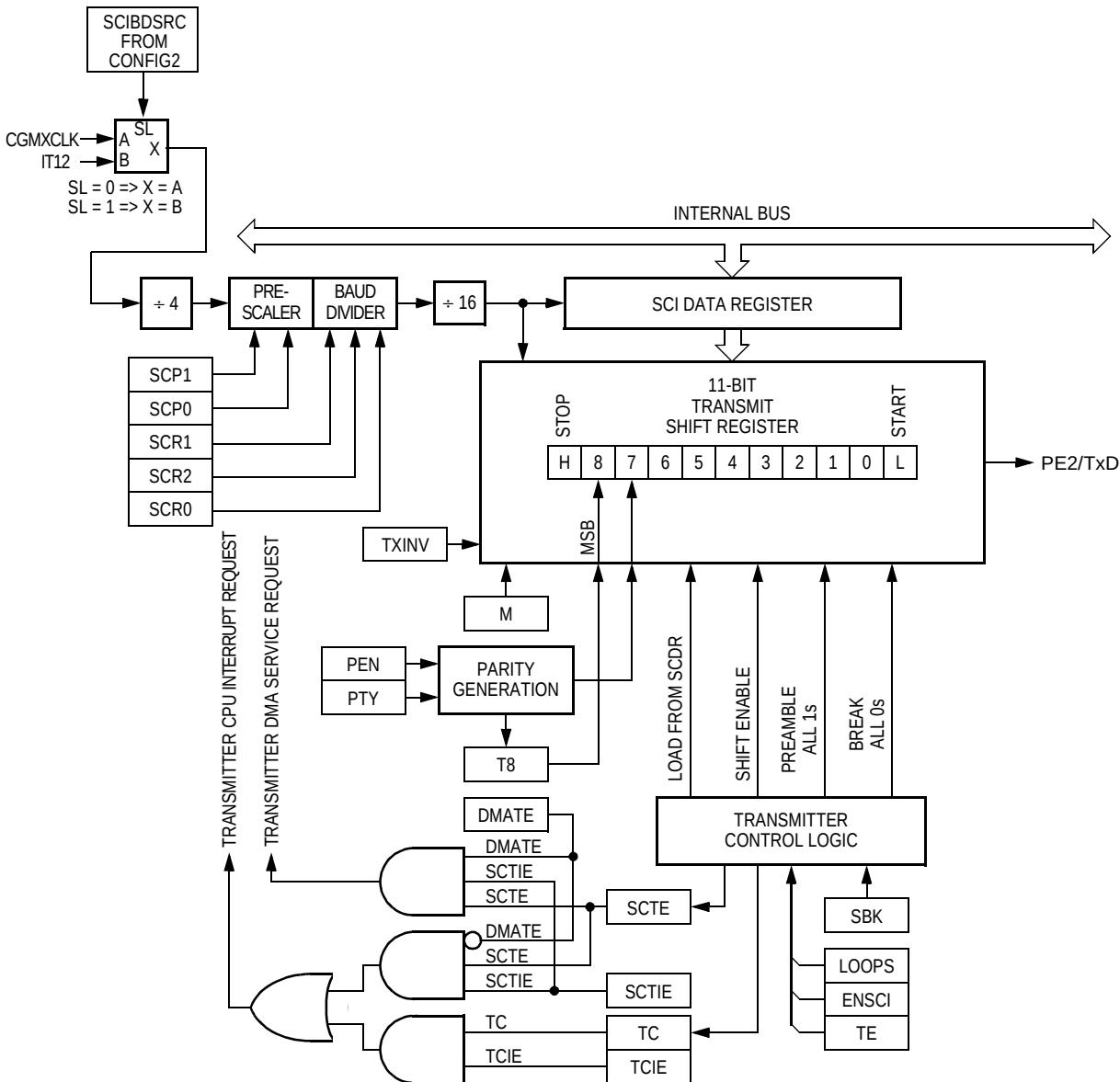
Figure 18-4. SCI Transmitter
