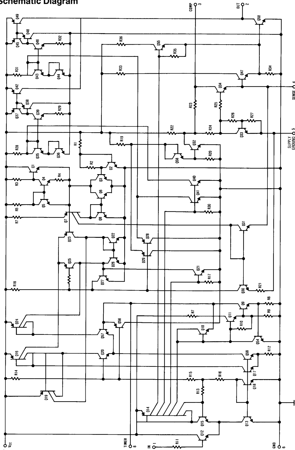
FIGURE 2. LM1949 Circuit
