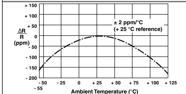
FIGURE 3 - TYPICAL TCR CURVE
