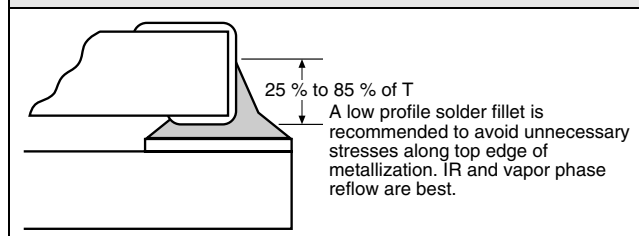
FIGURE 4 - RECOMMENDED MOUNTING 1)2)3)
