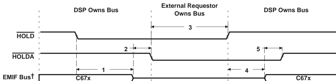
Figure 40. \overline{\text{HOLD}}/\overline{\text{HOLDA}} Timing
