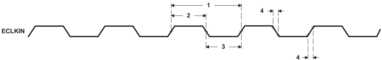
Figure 27. ECLKIN Timings
