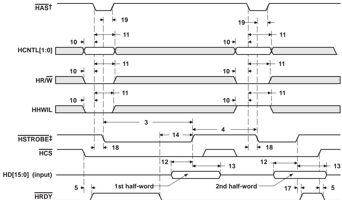
Figure 48. HPI Write Timing ( \overline{HAS} Used)
