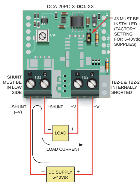
Figure 2A. Low-Side Shunt Connections for "-DC1" 5-40Vdc Non-Isolated Supply Models
