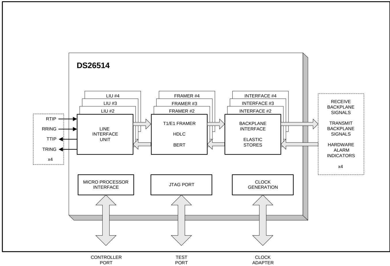
Figure 7-1. Block Diagram
