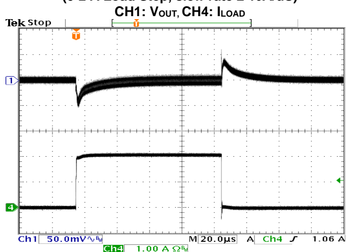
Transient Response at V_{IN} = 5\text{ V} V_{OUT} = 1.2\text{ V} , C_{OUT} = 1 \times 47\text{ }\mu\text{F} (0-2 A Load Step, slew rate \geq 10\text{ A}/\mu\text{S} )
