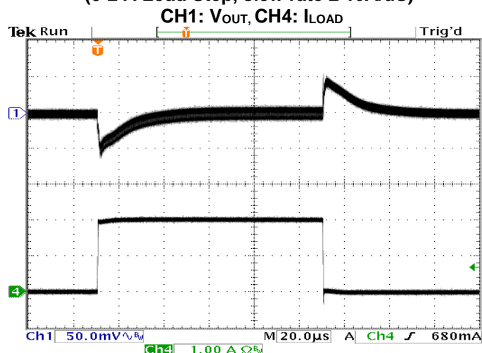
Transient Response at V_{IN} = 5\text{ V} V_{OUT} = 3.3\text{ V} , C_{OUT} = 1 \times 47\text{ }\mu\text{F} (0-2 A Load Step, slew rate \geq 10\text{ A}/\mu\text{S} )
