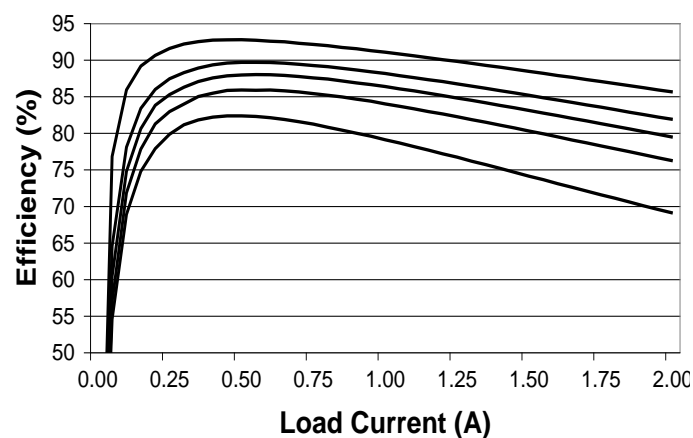
Efficiency vs. Load Current ( V_{in} = 3.3\text{V} )
