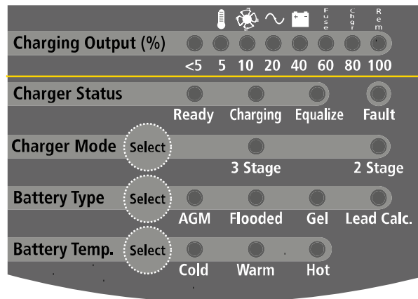
Figure 11 Onboard Display Panel
