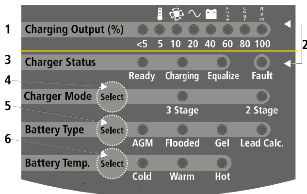
Figure 3 Onboard Control and Status Display Panel
