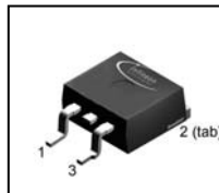
PG-TO263-3-2
